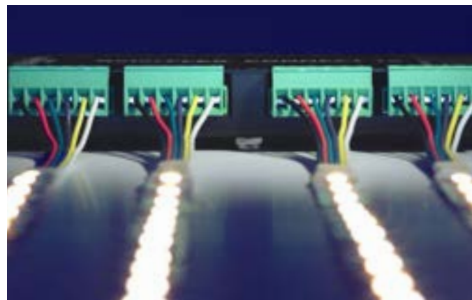
QolorFLEX Connect 10 uses 10 six position detachable Phoenix terminal block connectors to achieve a quick and well-ordered installation.
